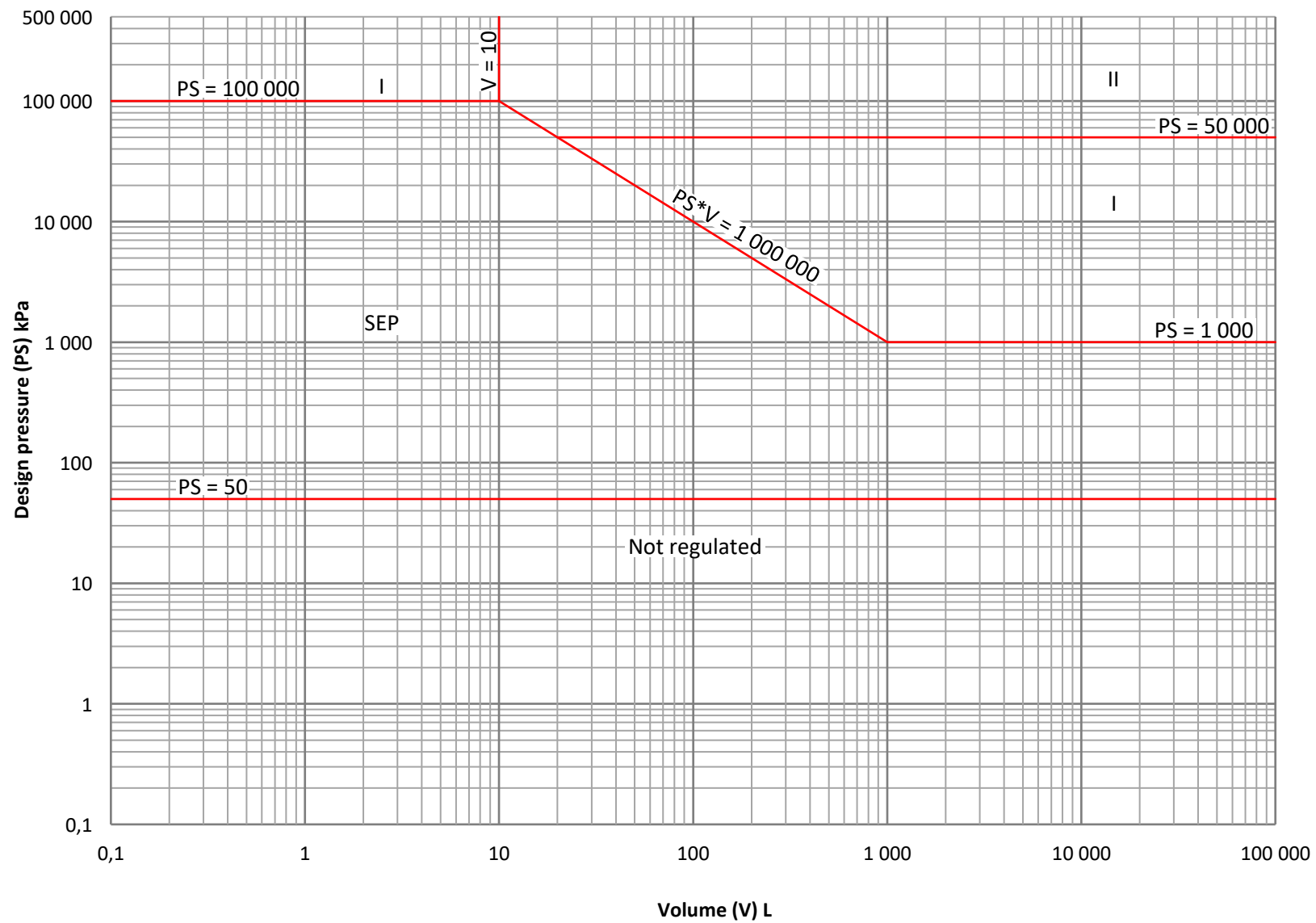
Figure 4 - Graph for vessels - Non-dangerous liquids
