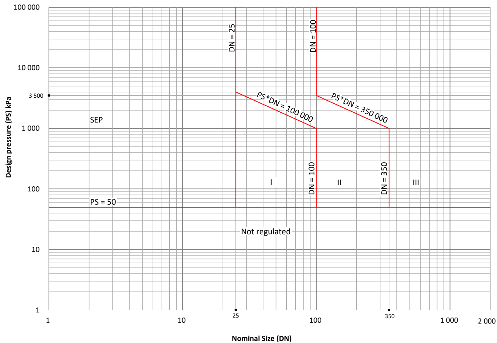
Figure 6 - Graph for piping - Dangerous gas
