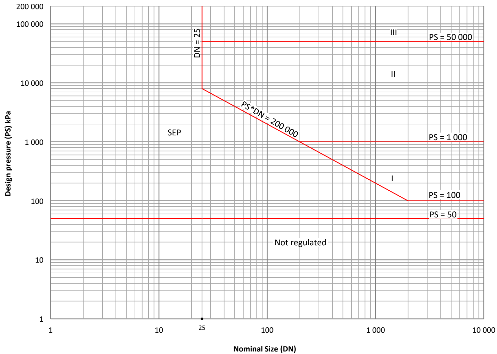
Figure 8 - Graph for piping - Dangerous liquids
