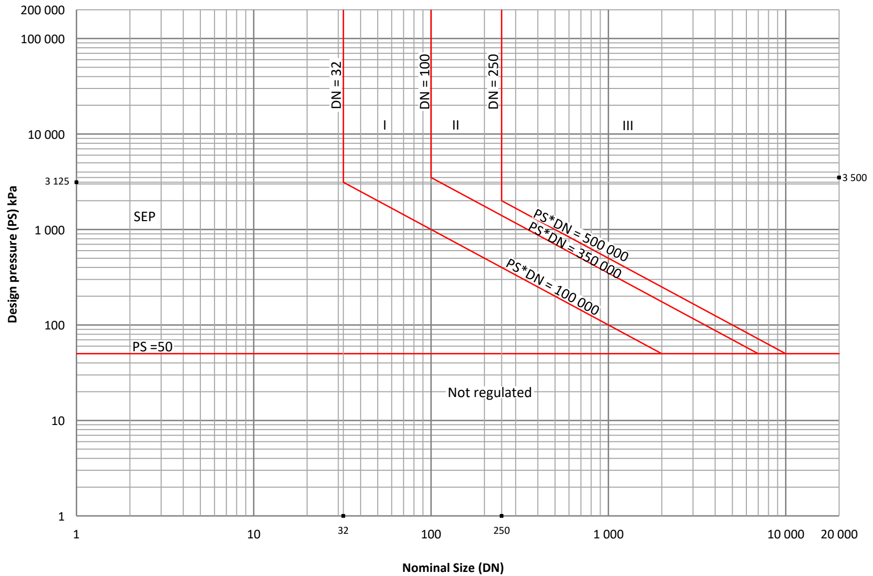
Figure 7 - Graph for piping - Non-dangerous gas
