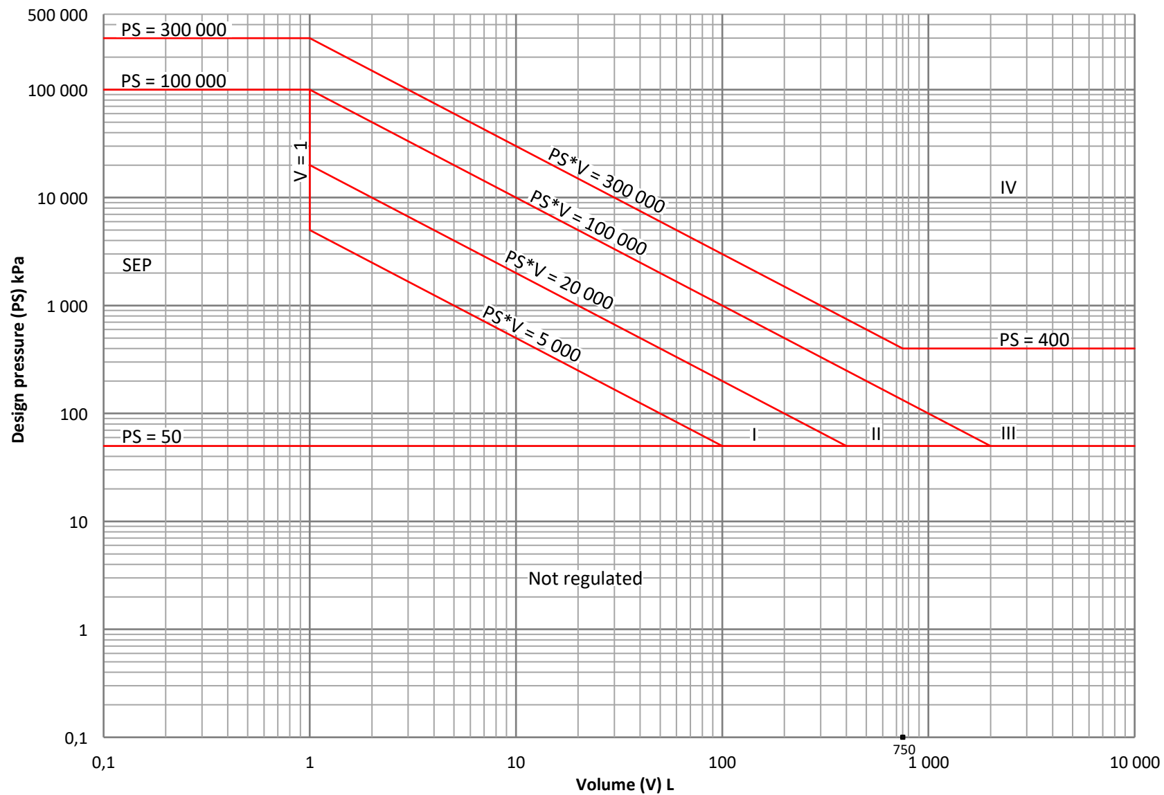
Figure 2 - Graph for vessels - Non-dangerous gas
