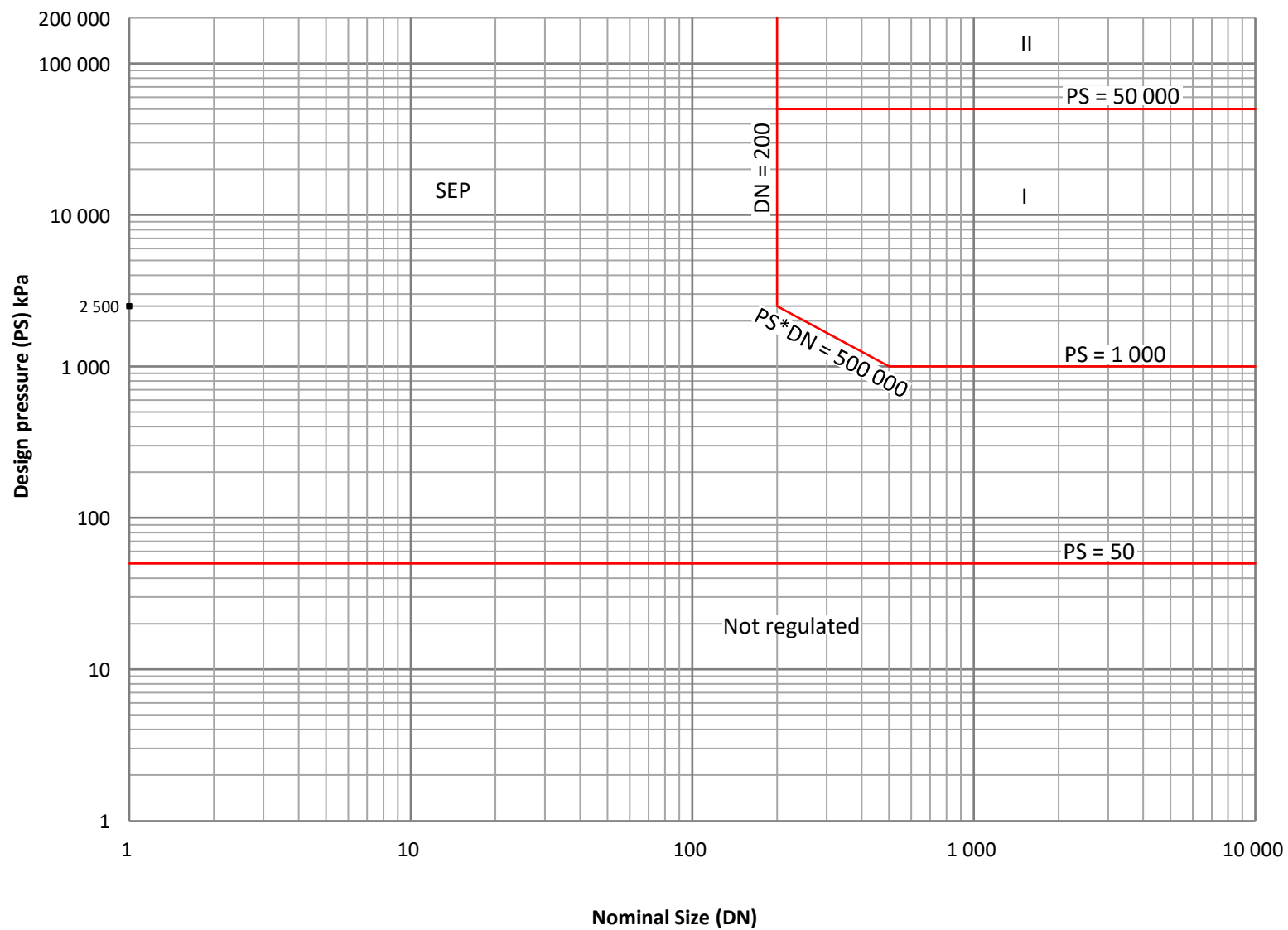
Figure 9 - Graph for piping - Non-dangerous liquids
