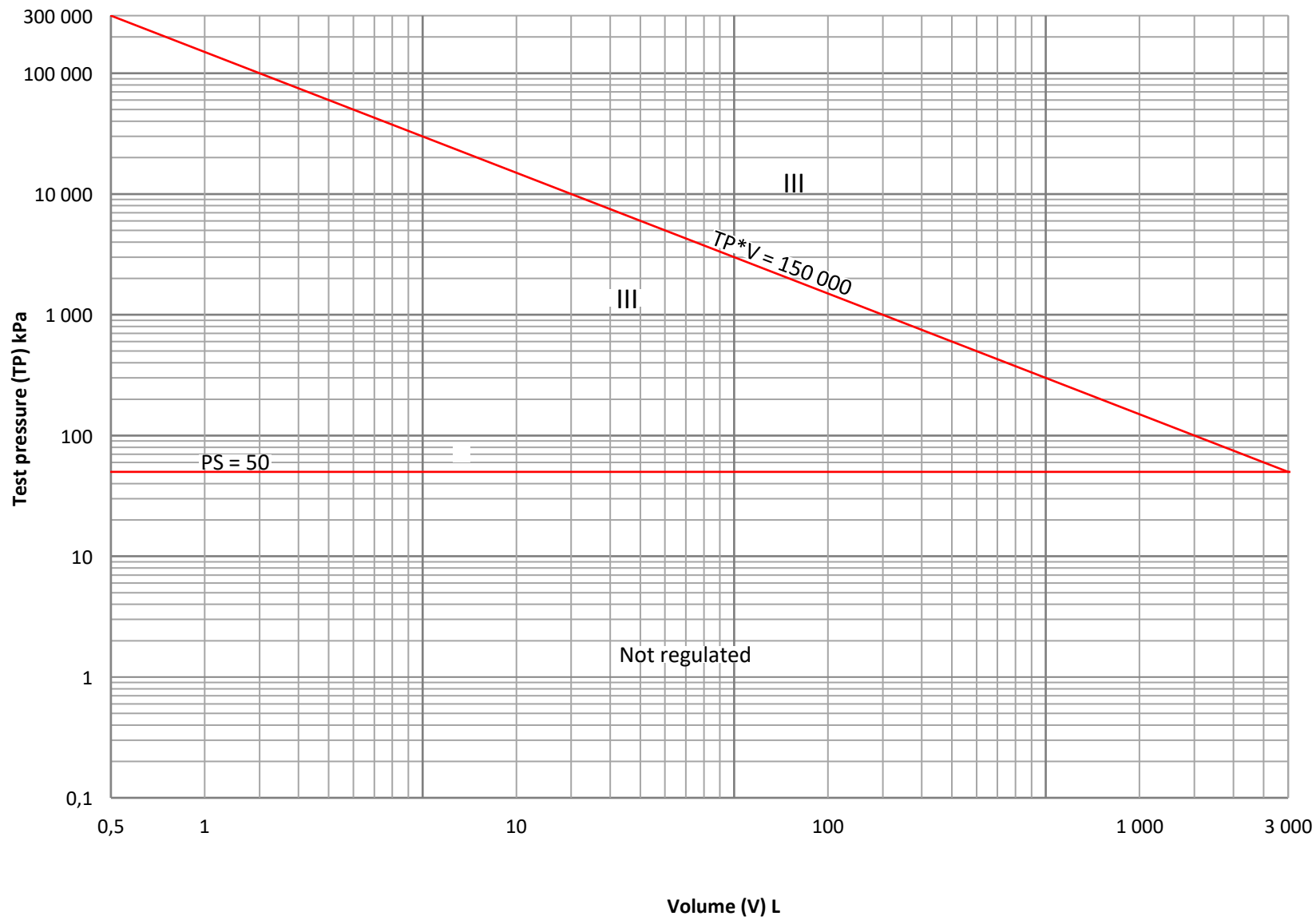
Figure 10 - Graph for transportable gas containers for all fluids
