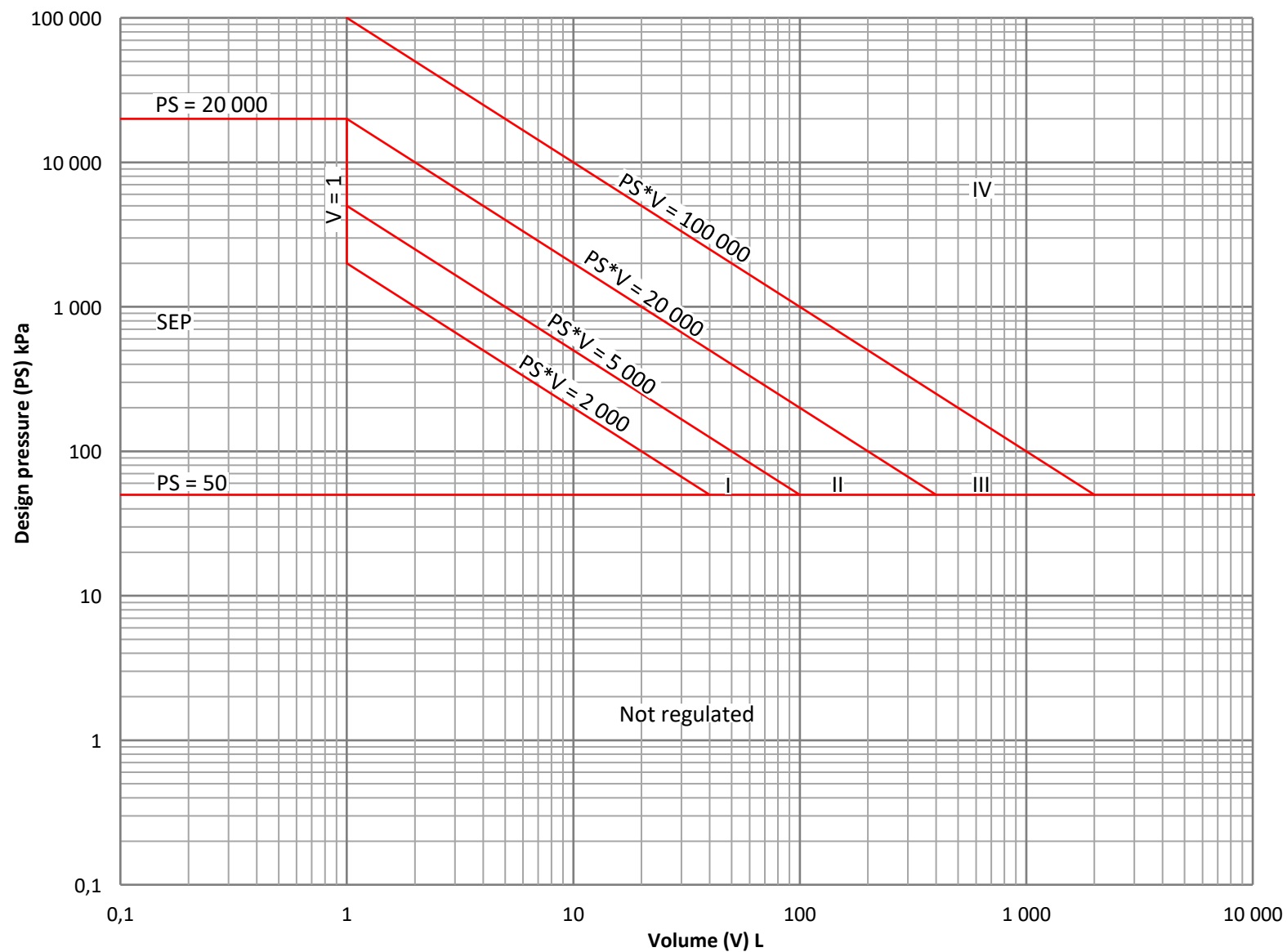
Figure 1 - Graph for vessels - Dangerous gas
