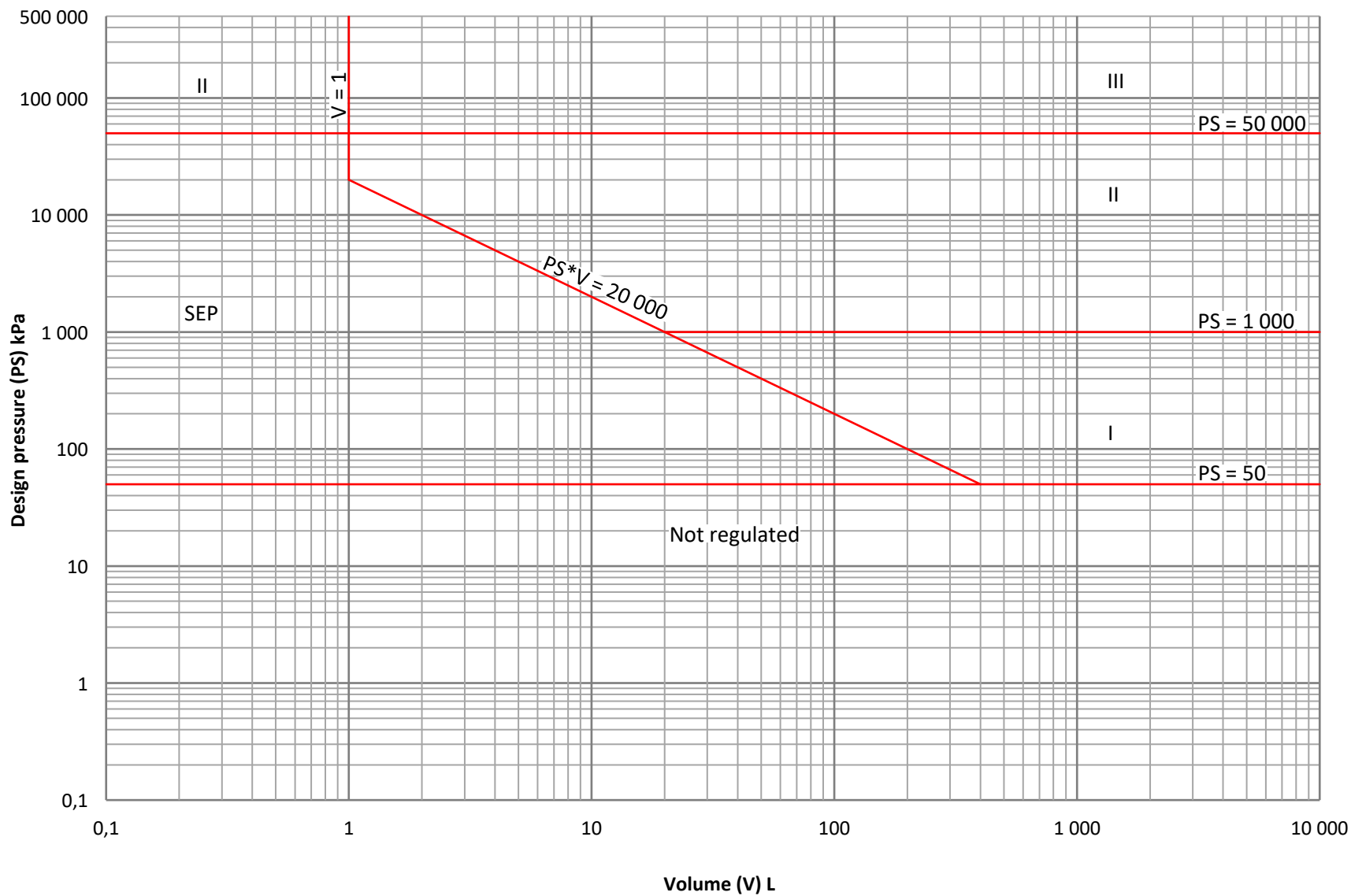
Figure 3 - Graph for vessels - Dangerous liquids
