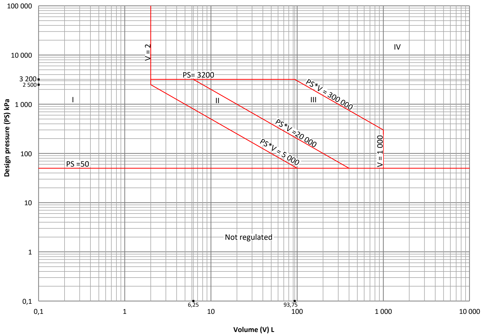
Figure 5 - Graph for steam generators
